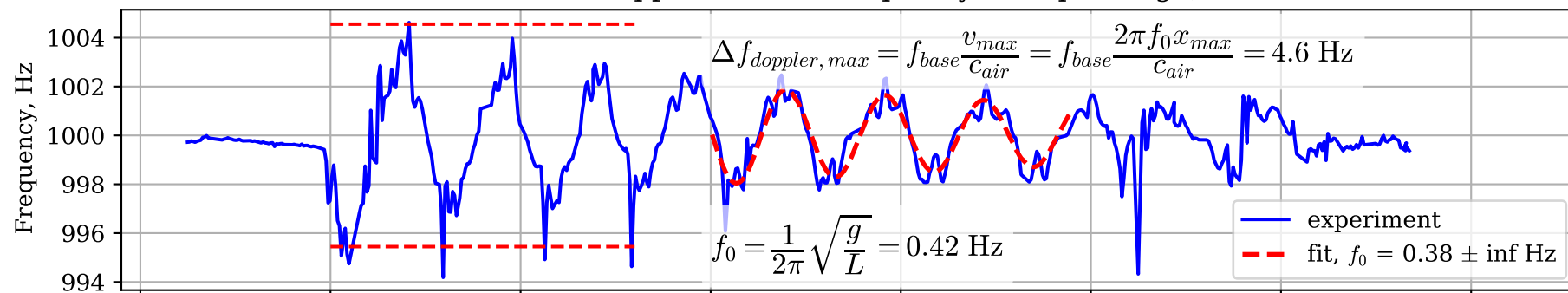
Pendulum Doppler effect : Frequency and speed(dg1).csv
