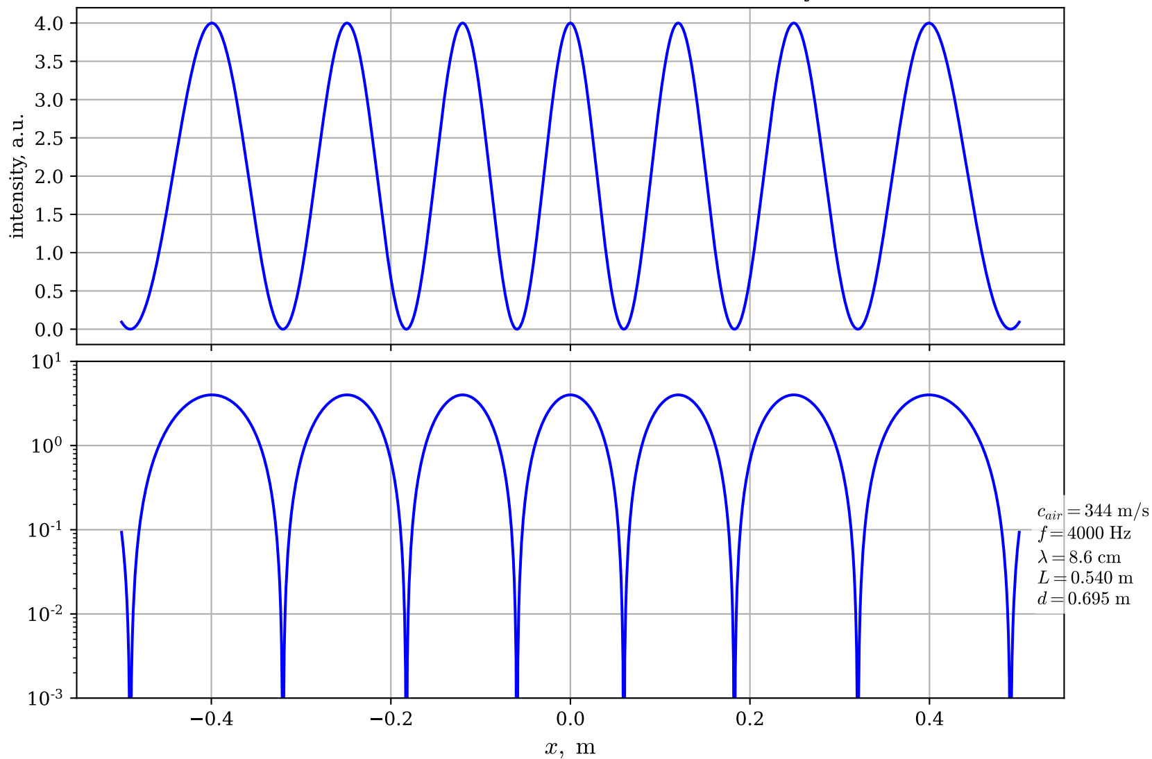
Interference of two acoustic sources (theory)
